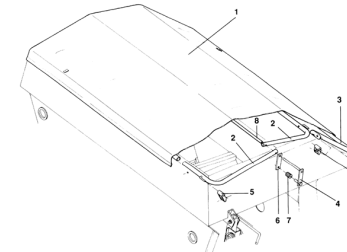
ETB-011813, Plandeka Jet 1503/04
